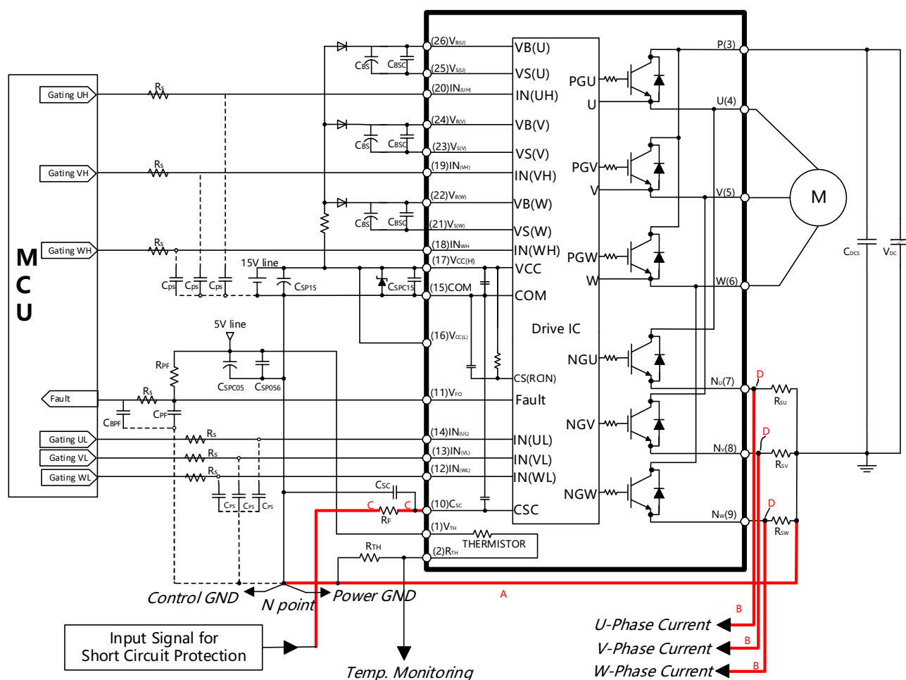
Figure 12 Application circuit
