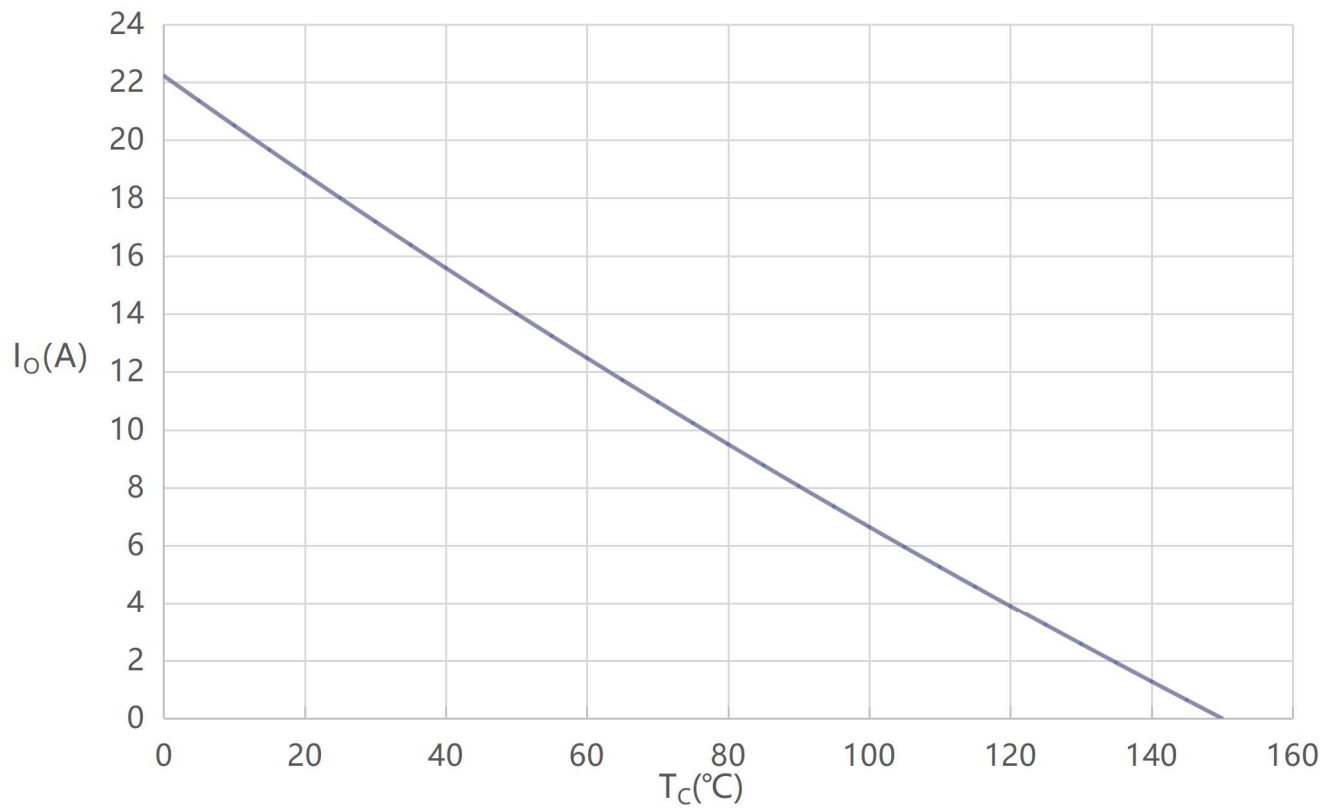
Figure 11 Maximum operating current SOA (Inverter Section)
