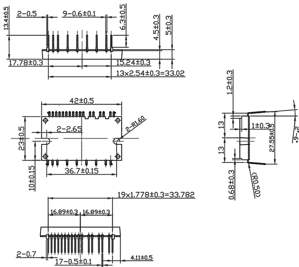
Figure 13 Package Outline
